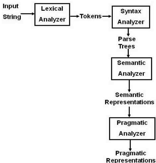
Figure 2: A Pipeline Architecture for Natural Language Processing
