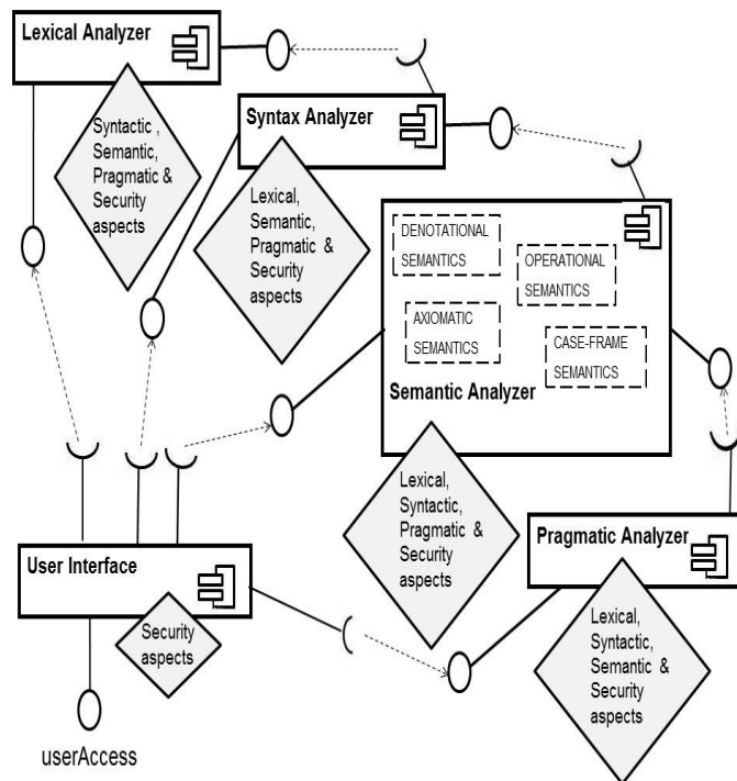
Figure 3. An Aspect Oriented Software Architecture for Natural Language Processing
